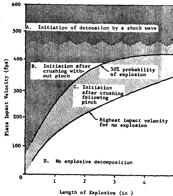
Fig. 21 Critical impact velocity as a function of explosive length, for 6-inch diameter 9404 PBX billets impacted by 6-inch diameter by 1-inch thick steel plates
